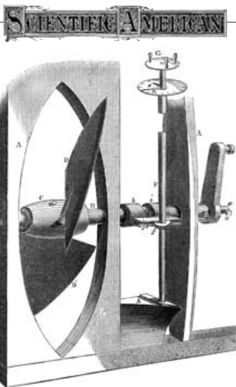
FEATHERING PROPELLER for ships, 1852
