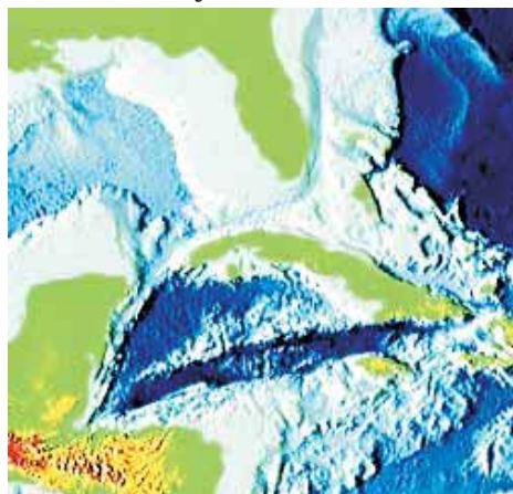
Satellite image of the Cayman Trough
