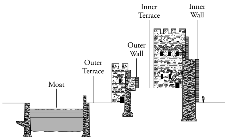
Cross section of the Theodosian Land walls
