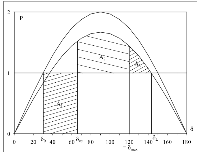
Figure 9.14. Criterion of areas and stability margin
