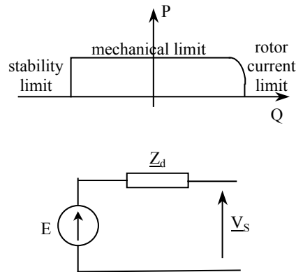
Figure 1.8. Diagram of a synchronous alternator
