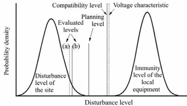
Figure 4.11. Illustration of the basic standardization concepts in power quality using time-dependent statistics concerning a site of the system where the real level (a) is estimated with a view to compare with the voltage characteristic and the real level (b) is estimated with a view to compare with the planning level
