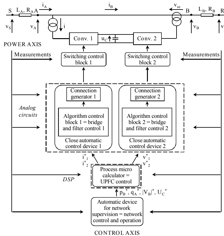
Figure 9.34. General diagram of hierarchical control of a UPFC
