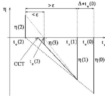
Figure 7.10. Schematic description of the search for a CCT. Adapted from [PAV 00]
