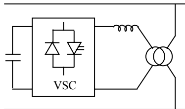
Figure 9.29. Flow diagram of a STATCOM or SVG, reactive power static compensator
