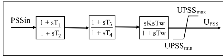
Figure 5.10. Structure of a “conventional” PSS controller
