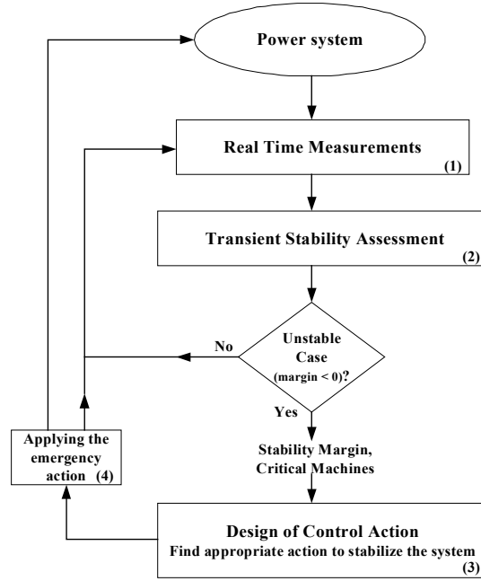
Figure 7.17. Organization of corrective assessment and control software in real time and in closed loop. Adapted from [ERN 00a]
