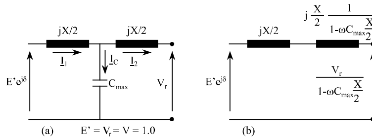
Figure 9.19. Circuit with fixed compensation of SVC type and corresponding Thévenin diagram
