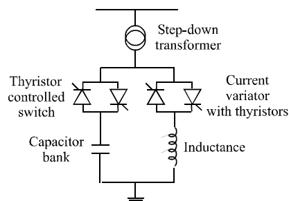
Figure 9.24. Flow diagram of an SVC
