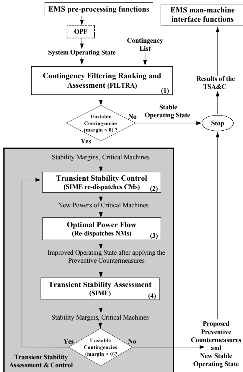
Figure 7.14. Integrated software for transient stability assessment and control in the preventive mode. Adapted from [PAV 00]
