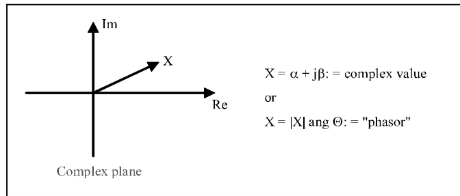
Figure 5.2. Notion of a “phasor”
