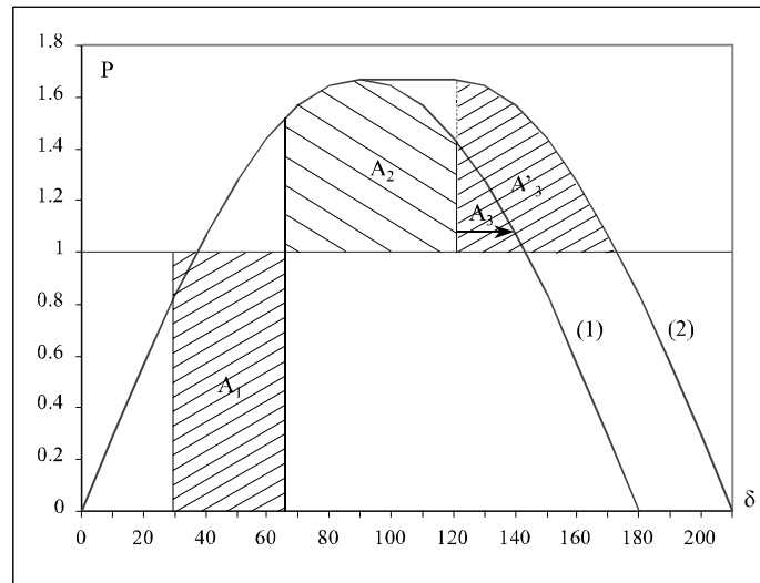
(1) without compensation, P = (V^2/X)\sin\delta (2) with compensation ( \alpha_{\max} = 30^\circ ), P = (V^2/X)\sin(\delta - \alpha)
