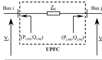
Figure 9.38. Model of two injections of power
