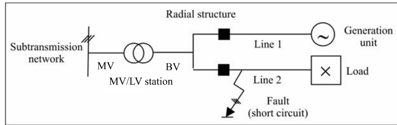
Figure 2.8. Influence of the decentralized production on the selectivity of the distribution network protection
