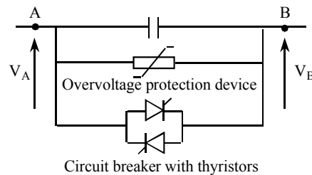
Figure 9.23. Diagram of the TSSC principle
