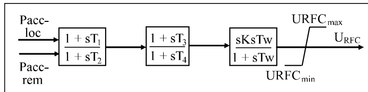
Figure 5.12. Double input RFC controller
