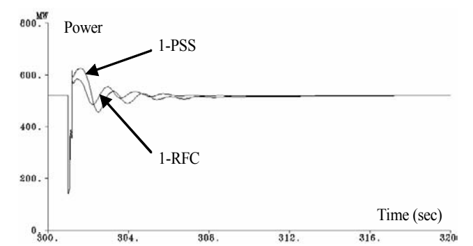
Figure 5.17. RFC against PSS, wheeling capacity at P_{wheeling} = 500 MW
