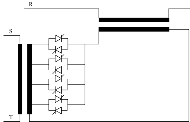
Figure 9.8. Phase shifting transformer with electronic switch
