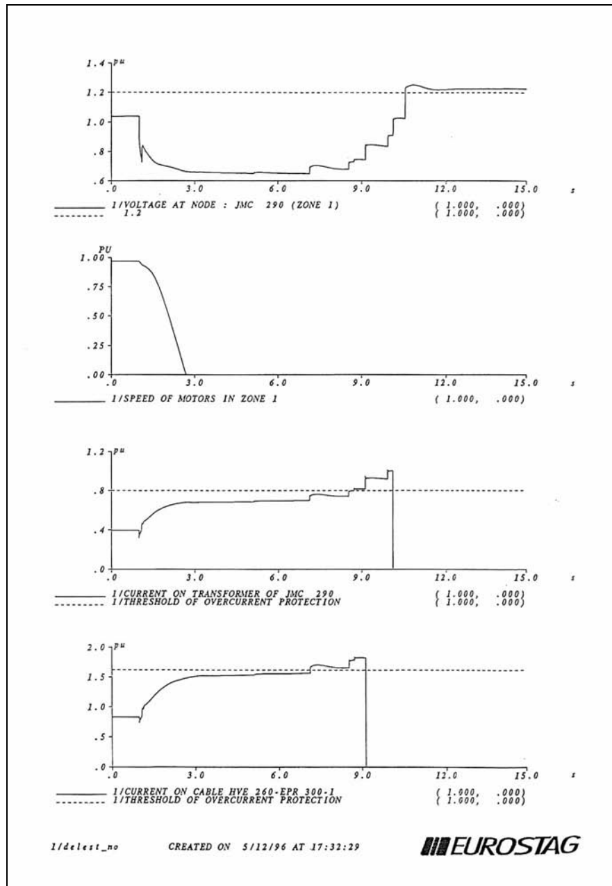
Figure 8.3. "Export" of the incident affecting zone 2 to zone 1
