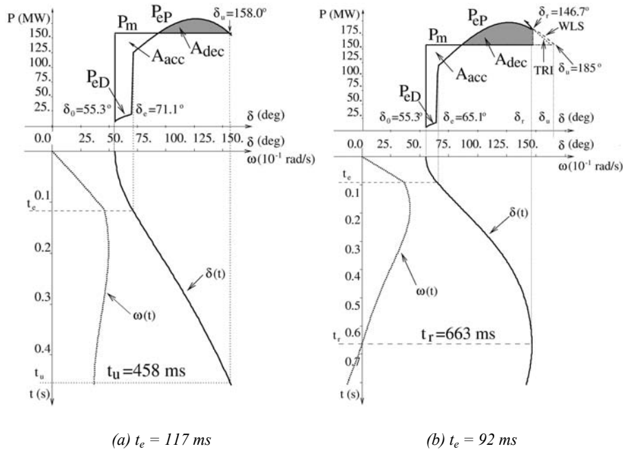
Figure 7.2. Time and P-\delta representations for the OMIB of the 3-machine system. Contingency no. 2. Adapted from [PAV 00]
