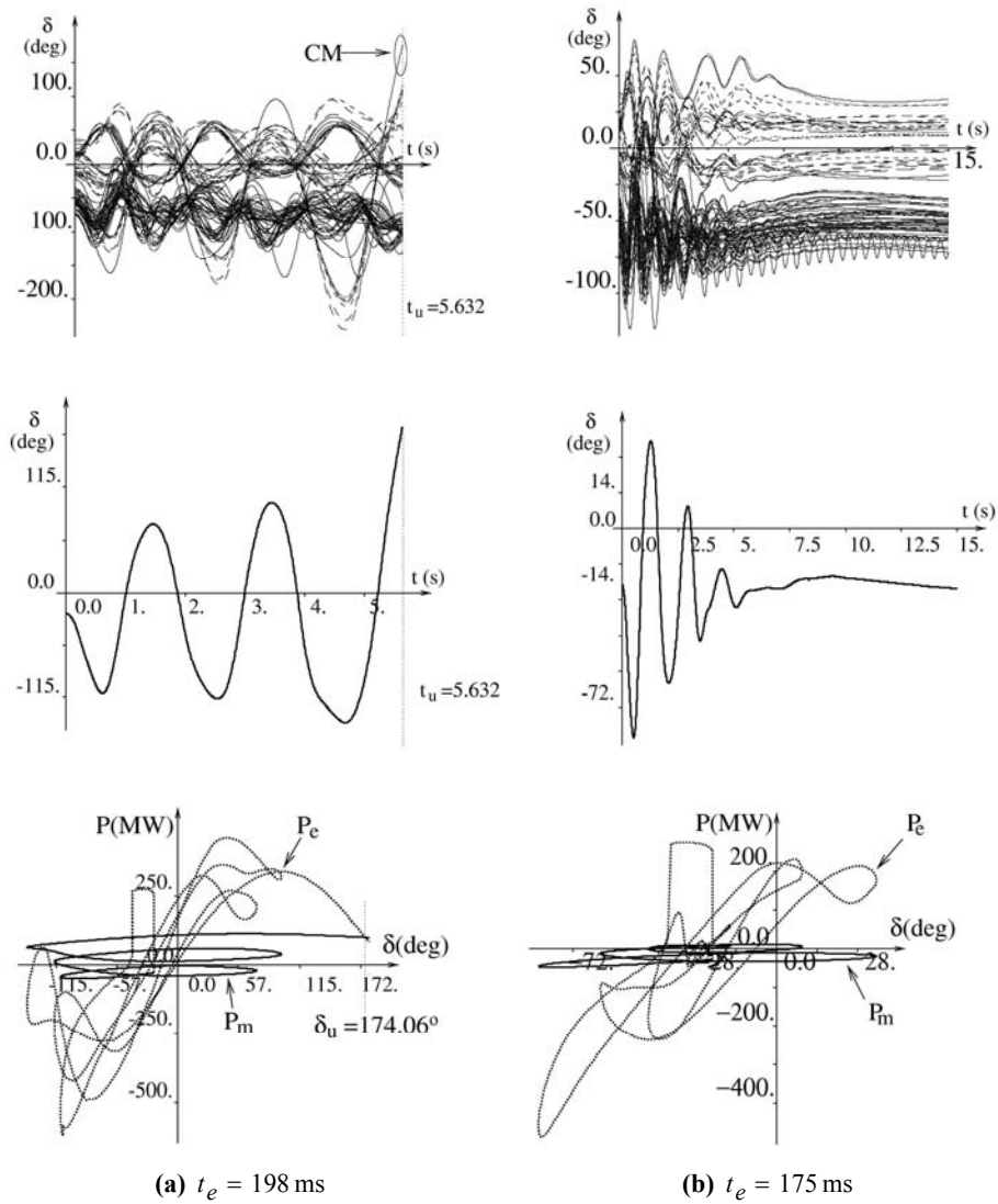
Figure 7.4. Three typical representations of back- and multi-swing phenomena simulated on the Hydro-Quebec system for two clearing times: one larger and one smaller than CCT
