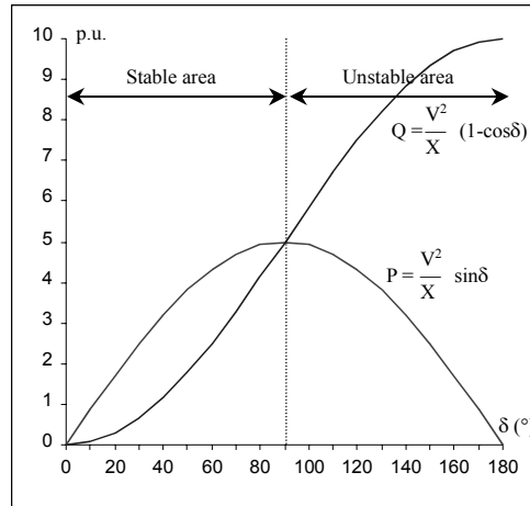
Figure 9.2. Variation of active and reactive power with transmission angle, for a link with reactance (see Figure 9.1 with V_a = V_b = 1.0 ; X = 0.2 )
