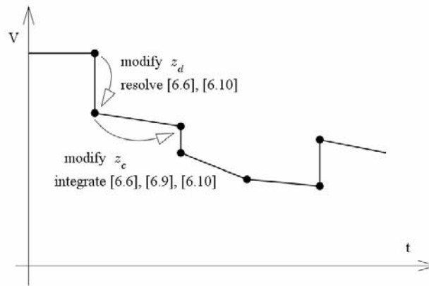
Figure 6.8. Quasi steady-state simulation
