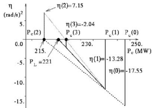
Figure 7.11. Schematic description of the search for a power limit. Adapted from [PAV 00]
