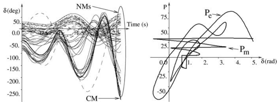
Figure 7.15. Loss of synchronism in “back- multi-swing mode”. South-southeast Brazilian power system, 56 machines, 1185 nodes. Contingency no. 159; t_c = 167 ms. Operating conditions of the base case. Adapted from [BET 99]
