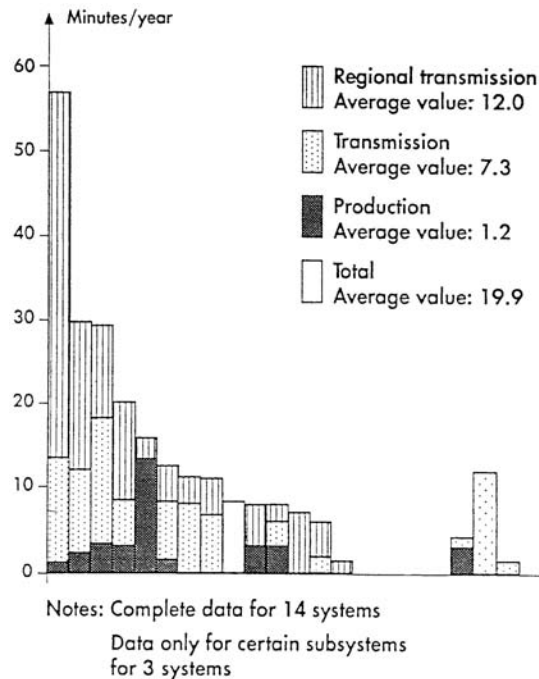
Figure 4.13. Statistics on AIT of 17 UNIPED member countries for the period 1982–1991
