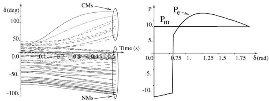
Figure 7.16. Loss of synchronism in “first-swing” inter-area mode. South-southeast Brazilian power system, 56 machines, 1185 nodes. Contingency no. 239; t_e = 167 ms. Operating conditions of the base case. Adapted from [BET 99]
