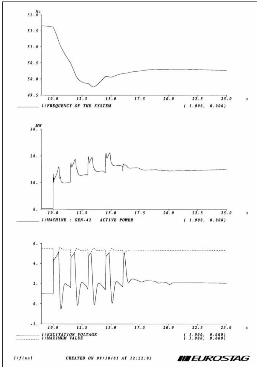
Figure 8.10. Start in waves of the driving load in an isolated network
