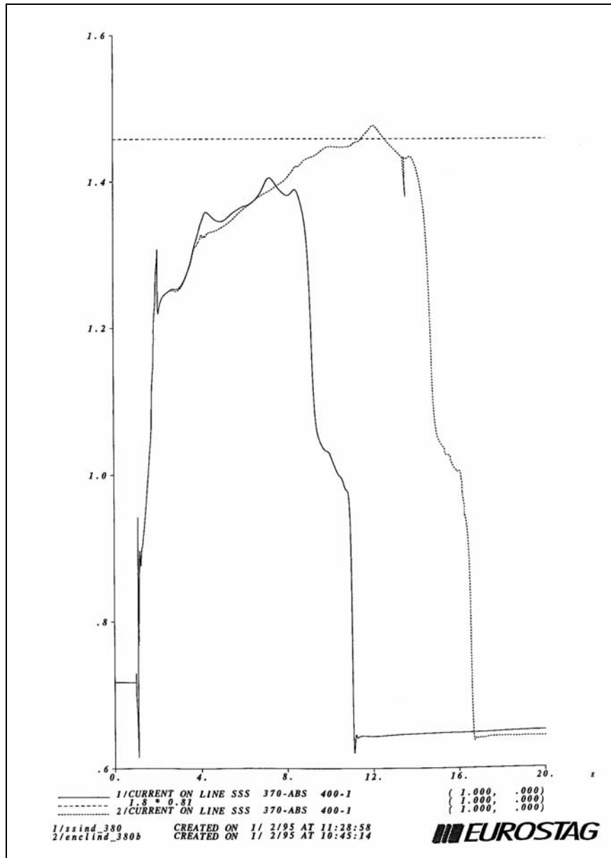
Figure 8.7. Influence of coordinated closing of shunt inductance on the evolution of line currents
