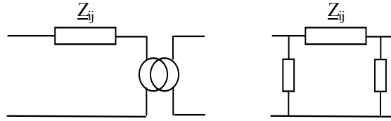
Figure 1.2. Equivalent circuit diagrams of transformer: (a) with ideal transformer, (b) through a \pi -diagram
