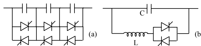
Figure 9.7. Series compensation (a: capacitors with electronic switches, b: system with controller)
