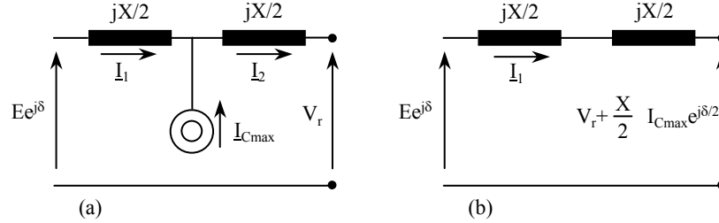
Figure 9.20. SVG in current limitation, general diagram and Thévenin diagram
