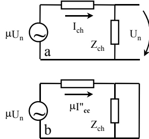
Figure 4.14. Increase in the short circuit current in a loaded network at a point where the voltage is equal to U_n ( \mu > 1 ); a) initial conditions in a loaded network, b) short circuit conditions
