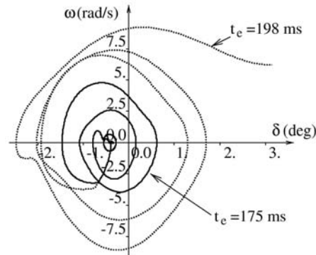
Figure 7.5. Phase plane of the OMIB. Representation of back- and multi-swing phenomena of Figures 7.4. Adapted from [PAV 00]
