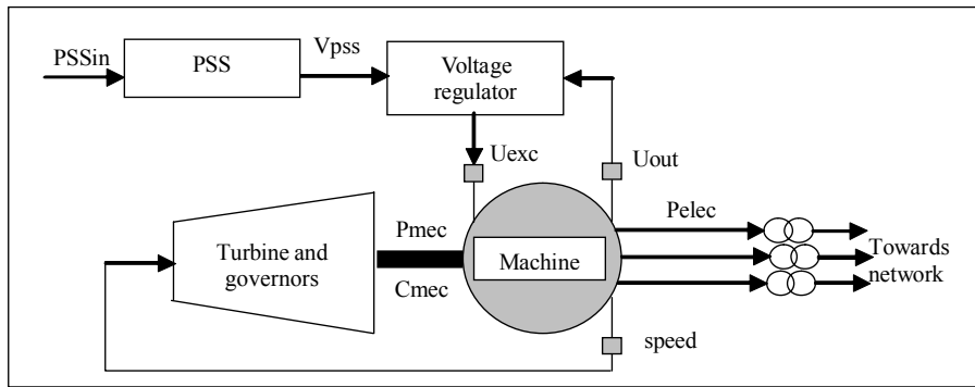
Figure 5.9. Overall structure of a machine connected to the network
