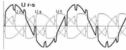
Figure 4.4. Commutation notches due to a three phase 3 rectifier (in addition their recurrence causes a permanent distortion)
