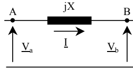
Figure 9.1. Single phase diagram of power exchange between two points linked by pure reactance X
