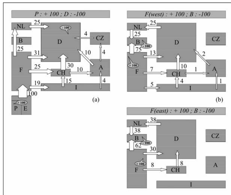
Figure 2.4. Power flow in the UCTE network between Portugal and Germany (a) and between France and Belgium (b)
