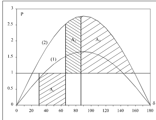
(1) without compensation, P = (V^2/X)\sin \delta (2) with compensation ( k = 0.4 ), P = (V^2/(1-k)X)\sin \delta
