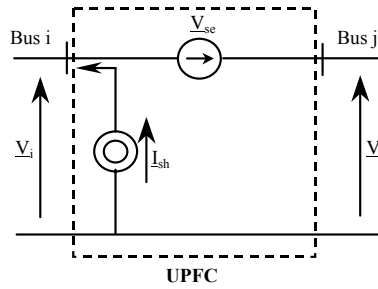
Figure 9.36. Model of series voltage source and shunt current source
