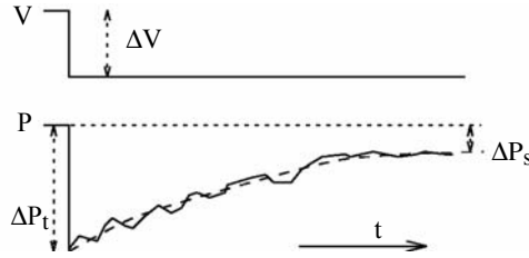
Figure 6.7. Response of power consumed to a voltage drop
