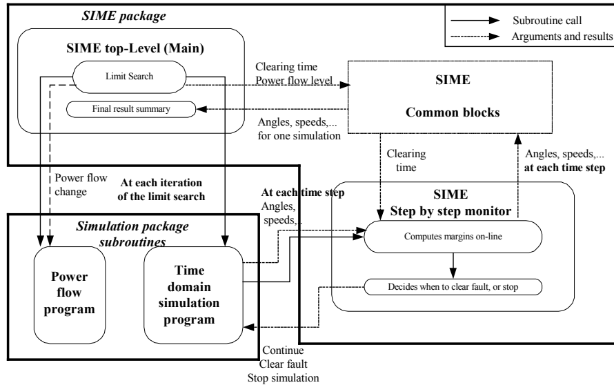
Figure 7.3. Coupling of SIME with a transient stability time domain program. Diagram of the principle. Adapted from [ERN 98c]
