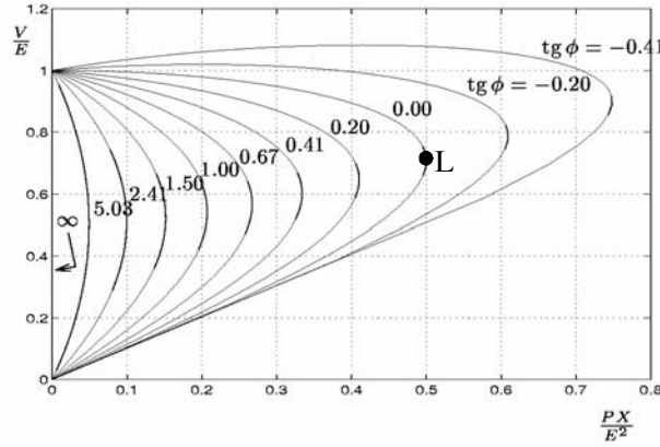
Figure 6.3. PV curves at constant power factor (referred to by the value of \text{tg } \phi )
