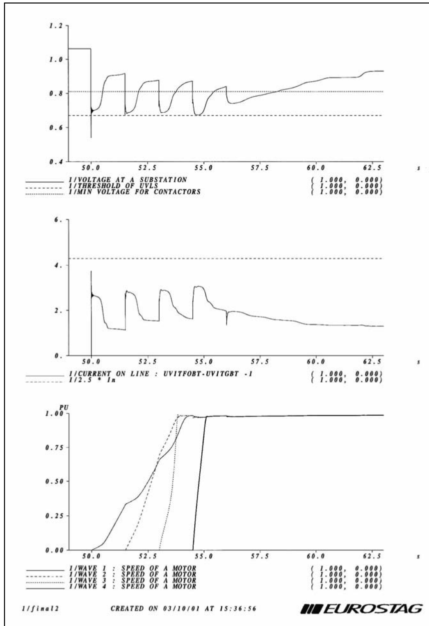
Figure 8.9. Start in waves of the driving load for an industrial site operating in an interconnected network
