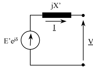
Figure 9.13. Simplified model of a synchronous machine in transients
