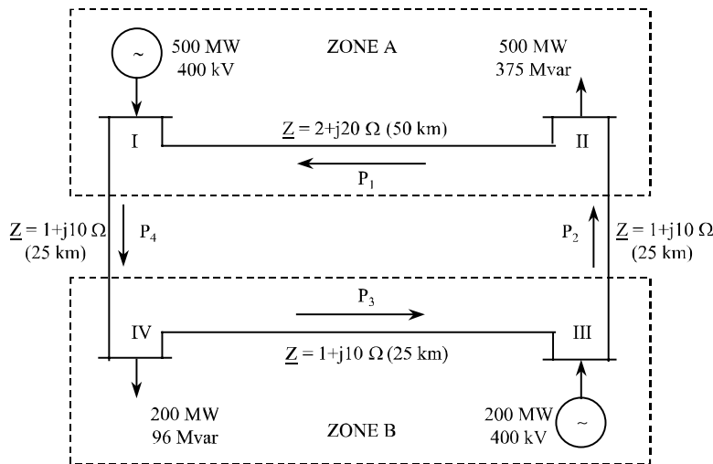
Figure 9.6. Basic meshed network
