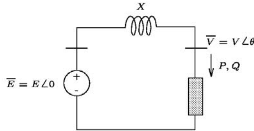
Figure 6.1. Simple generator-load system
