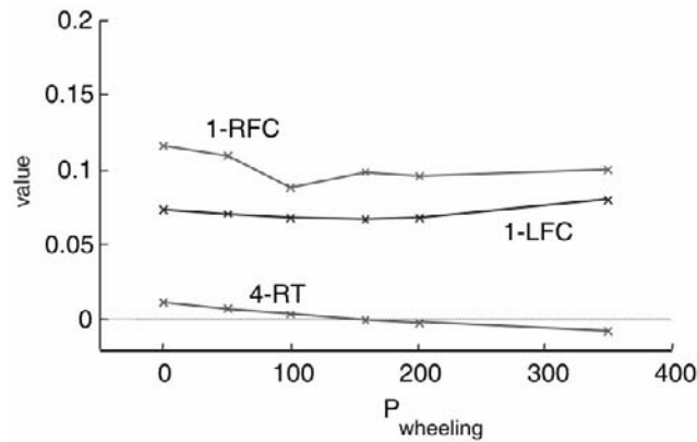
Figure 5.14. Damping factor migration for the nominal case for all the controllers
