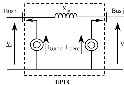
Figure 9.37. Model of two current sources
