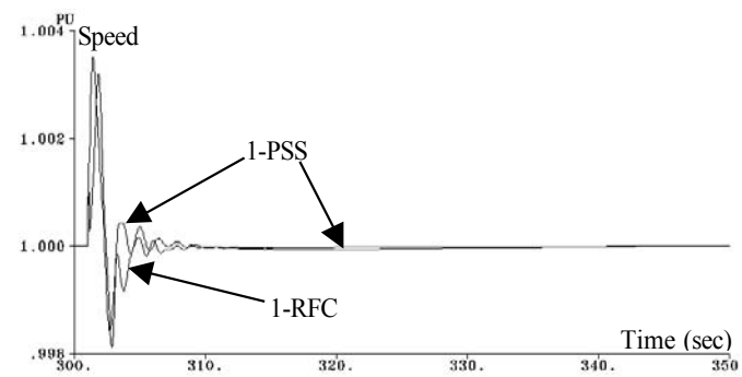
Figure 5.16. RFC against PSS, speed of machine 12 at P_{wheeling} = 500 MW
