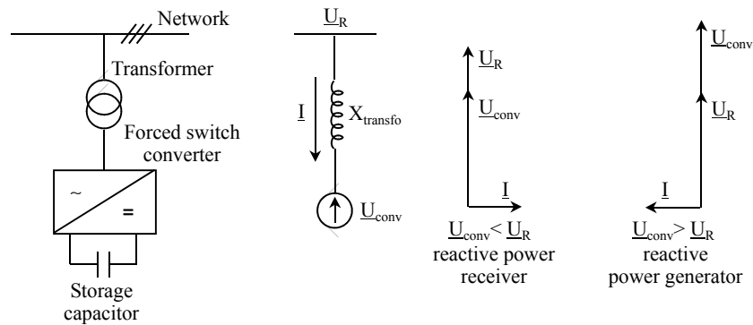
Figure 9.30. Operating principle of the advanced shunt static compensator, STATCOM
