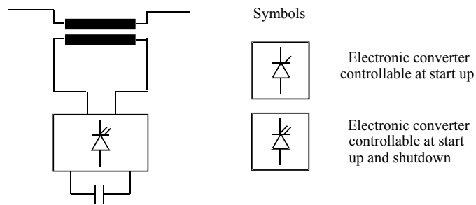
Figure 9.9. Series compensator with electronic converter
