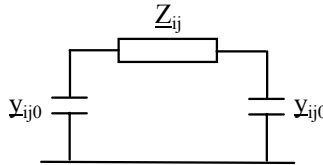
Figure 1.1. Equivalent circuit diagram of an electrical line
