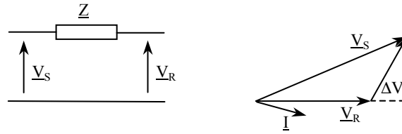
Figure 1.3. (a) Short line, (b) vector diagram
