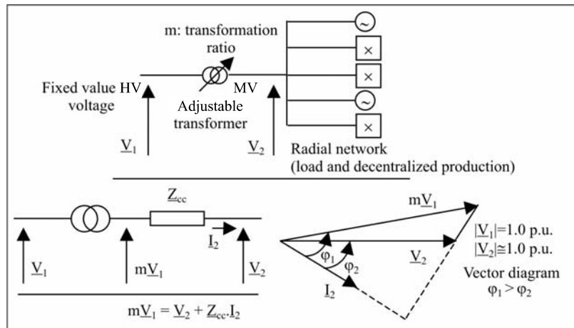
Figure 2.9. Connection of decentralized production to the distribution network (MV), effects of supply from a substitute power
