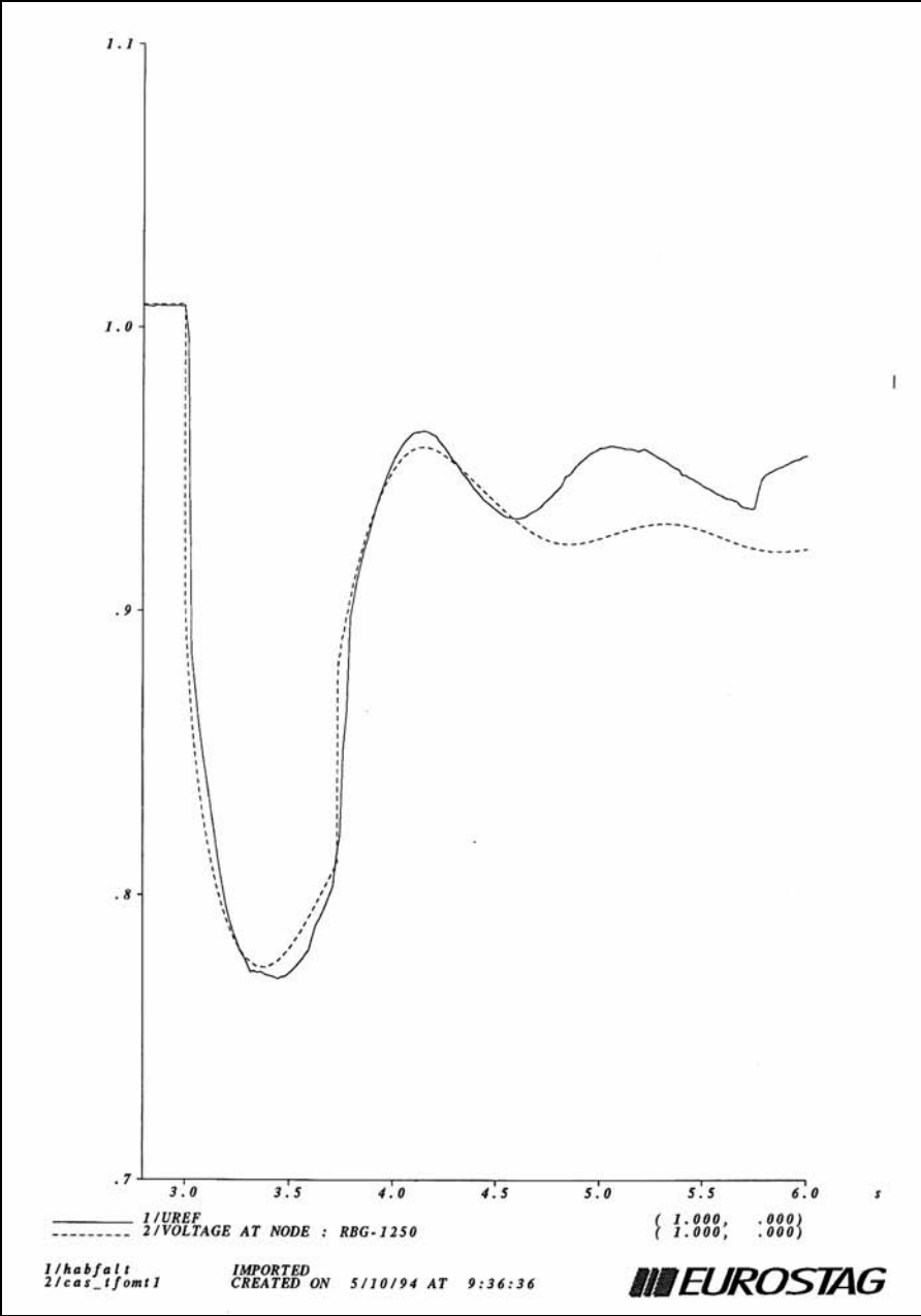
Figure 8.5. Comparison of measured and simulated voltage
