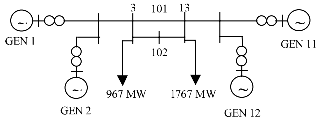
Figure 5.8. 4-machine test system [KUN 94]
