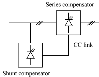
Figure 9.12. Unified power flow controller (UPFC)
