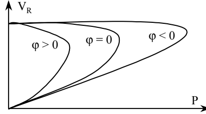
Figure 1.6. Power limit as a function of \varphi
