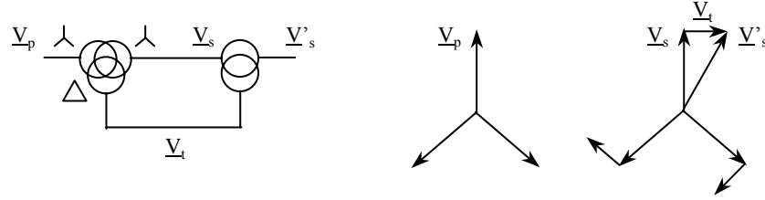
Figure 1.5. Diagram of the principle of the phase shifting transformer
