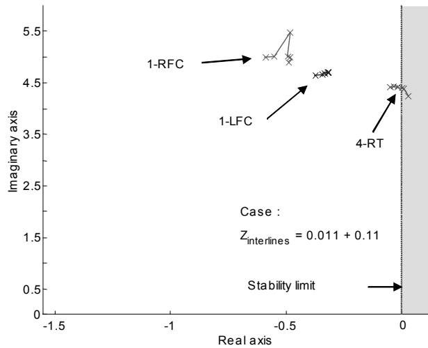
Figure 5.13. Eigenvalues for nominal case, all the controllers
