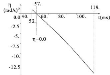
Figure 7.9. Variation of the stability margin with the disturbance clearing time and the OMIB mechanical power. 627-machine system. Adapted from [PAV 00]
