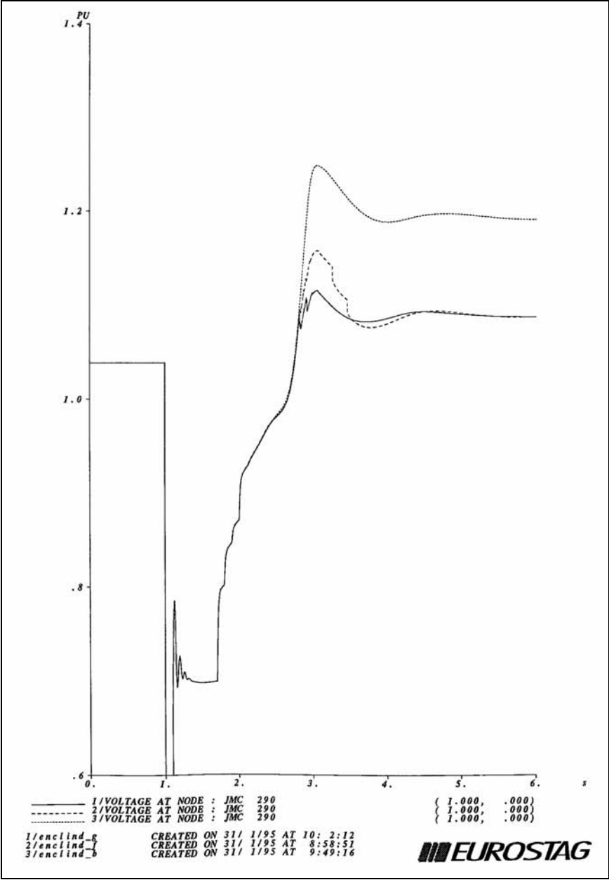
Figure 8.6. Comparison of responses of different implementations of load shedding plan
