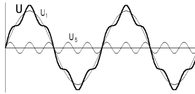
Figure 4.7. Distortion caused by only one harmonic ( h = 5 )
