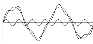
Figure 4.8. Distortion caused by a single interharmonics ( h = 3.5 )
