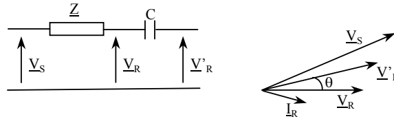
Figure 1.7. Principle of series compensation
