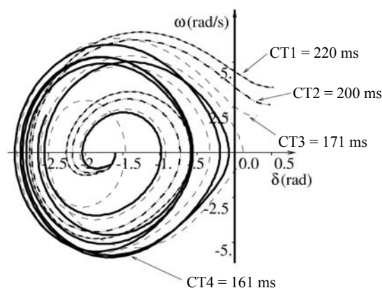
Figure 7.7. Phase plane of OMIB. Representation of back- multi-swing phenomena of Figures 7.6. Adapted from [PAV 00]
