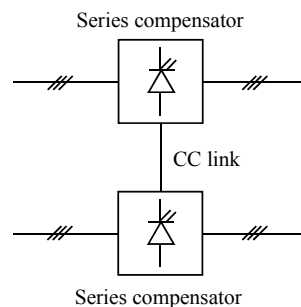
Figure 9.11. Interline power flow controller (IPFC)
