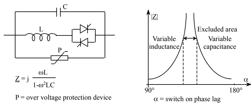
Figure 9.26. Flow diagram of the series compensator with parallel resonance circuit and control characteristic (ASC or TCSC)
