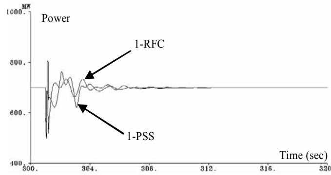
Figure 5.15. RFC against PSS, Pelec of machine 12 at P_{wheeling} = 500 MW
