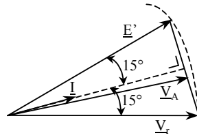
Figure 9.16. Vector diagram related to the system operation before the fault in the circuit in Figure 9.15
