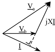
Figure 9.4. Vector diagram for V_a \neq V_b
