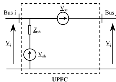
Figure 9.35. Model of two voltage sources
