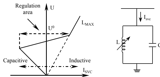
Figure 9.25. Control characteristic of an SVC
