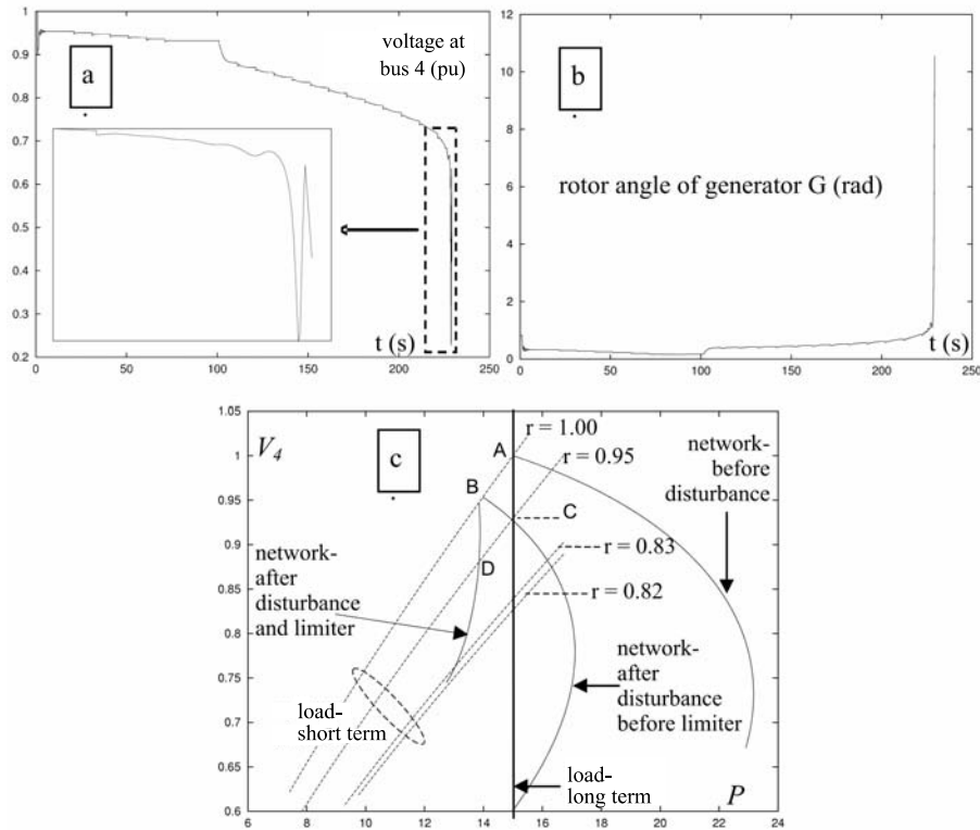
Figure 6.6. Example, 2 nd scenario: time evolutions and PV curves
