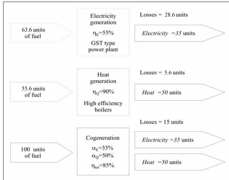
Figure 2.5. Comparison between a cogeneration unit and separate production
