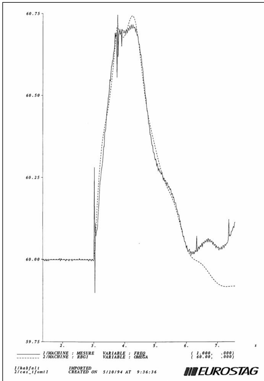
Figure 8.4. Comparison of measured and simulated frequencies
