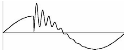
Figure 4.6. Dampened transient oscillation due to switching on of a capacitor bank
