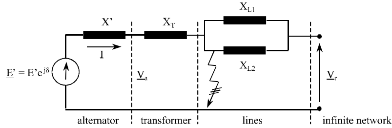
Figure 9.15. Single phase diagram in transient of an alternator connected to the network
