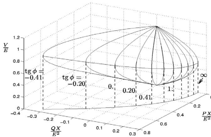
Figure 6.2. Voltage load based on active and reactive power consumed
