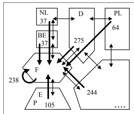
Figure 2.2. Exchanges in the UCTE network, following a 1,000 W power generation loss in France
