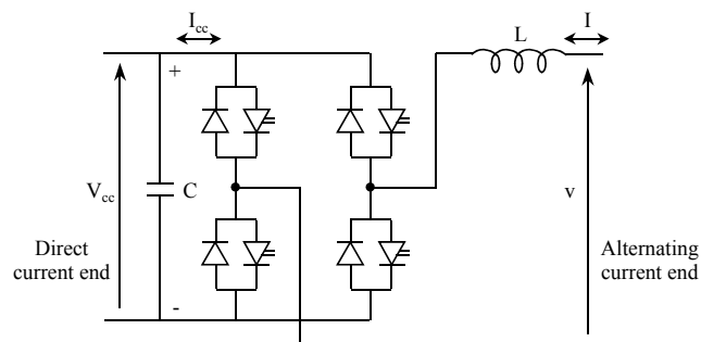
Figure 9.27. Flow diagram of a single phase voltage-sourced converter
