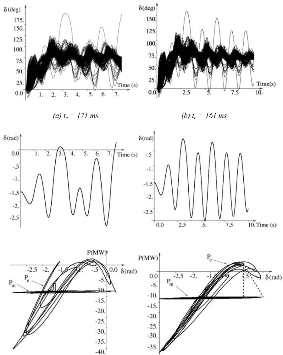
Figure 7.6. Three representations - type of back-multi-swing phenomena simulated on test system A of EPRI (627 machines). CCT(SIME) = CCT(ETMSP) = 168 ms. Adapted from [PAV 00]
