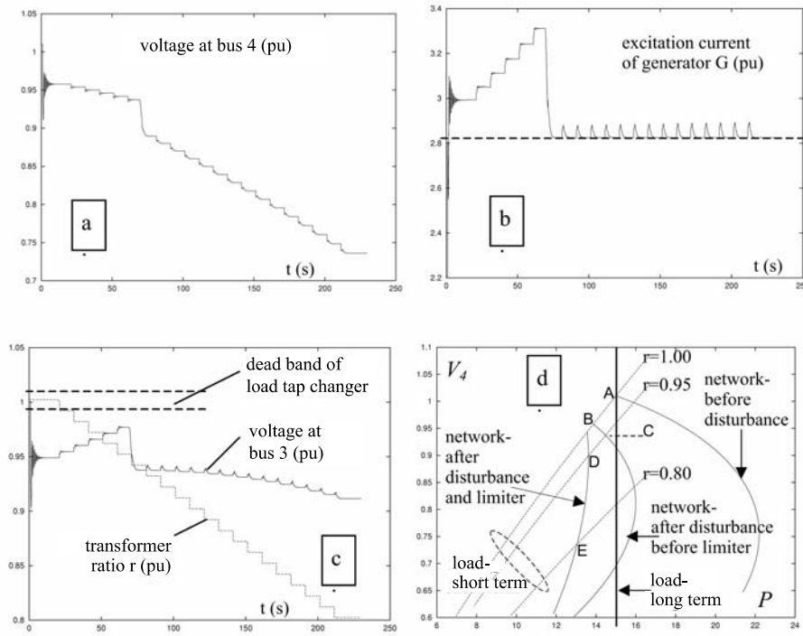
Figure 6.5. Example, 1 st scenario: time evolutions and PV curves
