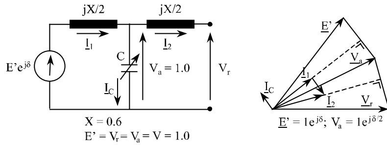
Figure 9.18. Diagram with shunt compensator and corresponding vectorial diagram
