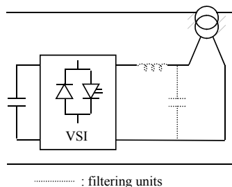
Figure 9.31. Flow diagram of a series compensator with converter, ASC or SSSC
