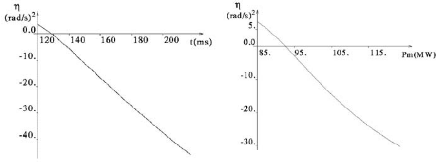
Figure 7.8. Variation of the stability margin with the disturbance clearing time and the OMIB mechanical power. 3-machine system. Adapted from [PAV 00]
