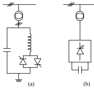
Figure 9.10. (a) Reactive power static compensator with controller, (b) static compensator with converter
