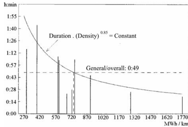
Figure 4.12. Unavailability of supply (min/customer per year), related to the load density (MWh per km of MV network) for ten distribution zones
