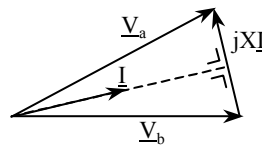
Figure 9.3. Vector diagram for V_a = V_b
