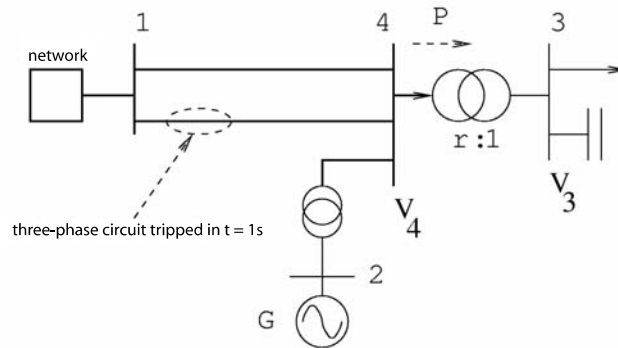
Figure 6.4. Single-line system diagram in the example
