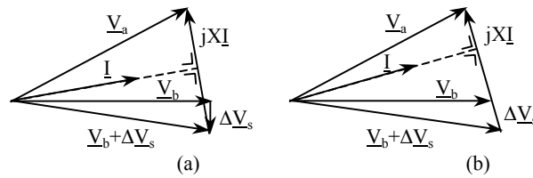
Figure 9.5. Influence of injection of additional voltage \Delta V_s to one of the extremities of the link (a: \Delta V_s in quadrature with V_b ; b: \Delta V_s in quadrature with I )
