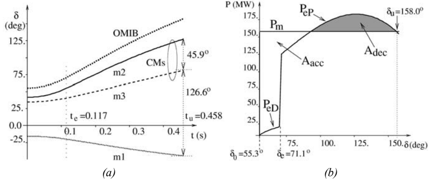
Time evolution of the machines and OMIB
