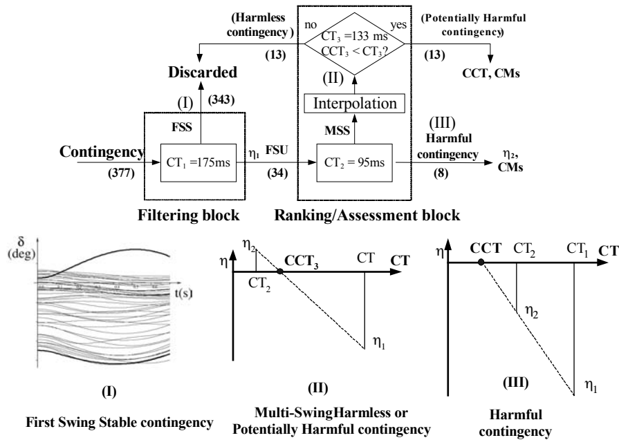
Figure 7.12. A construction of FILTRA. Schematic description of the different classes of contingencies. The numeric values in parenthesis correspond to a simulation carried out on the Hydro-Quebec system and indicate the number of contingencies classified in each of the categories. Adapted from [PAV 00]
