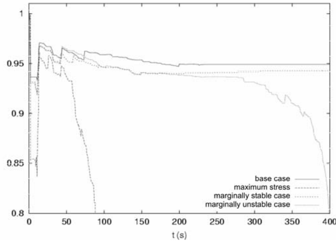
Figure 6.11. Evolution of voltage (in pu) for 4 stress levels of a binary search; Hydro-Quebec system
