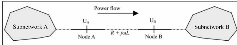
Figure 5.1. Transmission line model for power transfers
