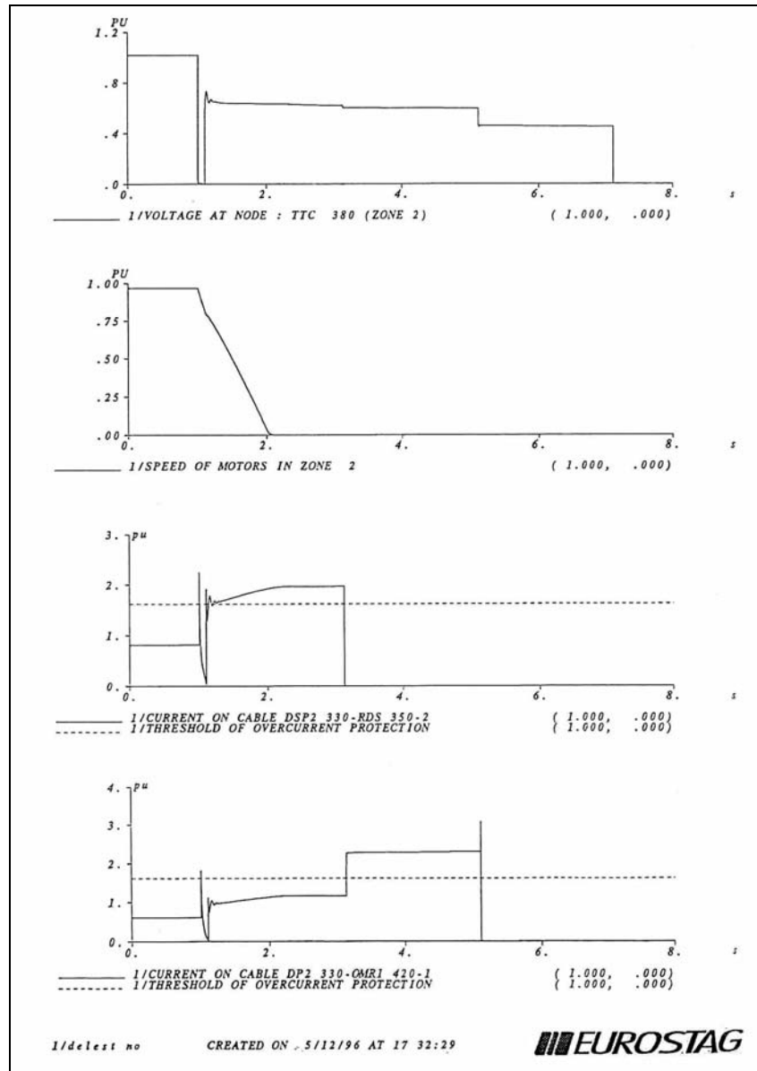
Figure 8.2. Simulation of a short circuit affecting zone 2
