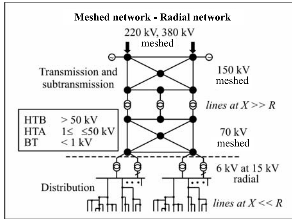
Figure 2.1. Meshed and radial structures of the networks
