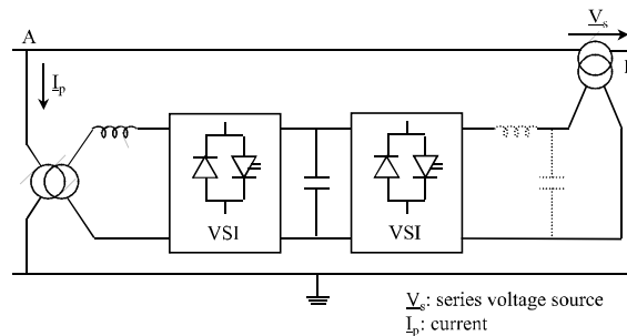
Figure 9.32. Flow diagram of the unified power flow controller, UPFC
