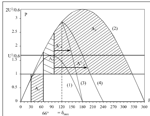
(1) without compensation (3) compensation with limitation ( \delta_{max} = 120^\circ ), type SVC (2) ideal compensation (4) compensation with limitation ( \delta_{max} = 120^\circ ), type SVG
