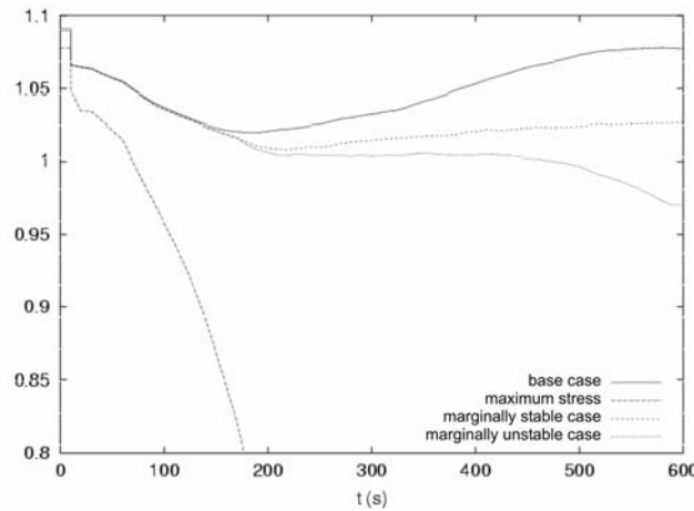
Figure 6.10. Evolution of voltage (in pu) for 4 stress levels of a binary search; RTE system
