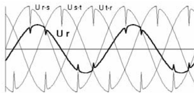
Figure 4.5. Commutation notches due to a three phase controller (in addition their recurrence causes a permanent distortion)
