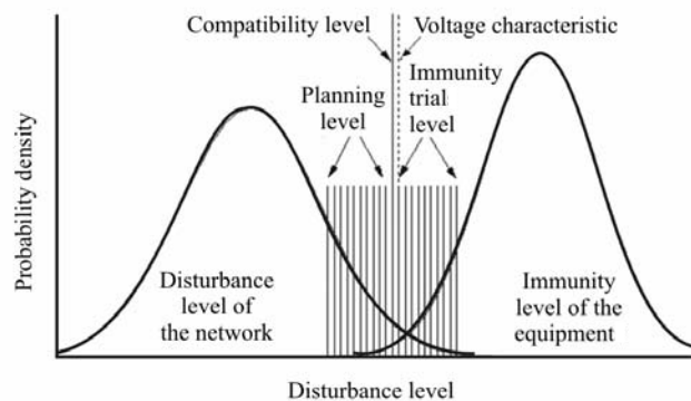
Figure 4.10. Illustration of the basic standardization concepts in power quality using time/place dependent statistics concerning the entire system
