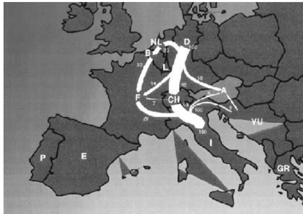
Figure 2.3. Flow of 100 MW power in the UCTE network from Germany to Italy
