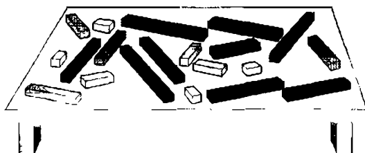
FIGURE 19: Cuisenaire rods
