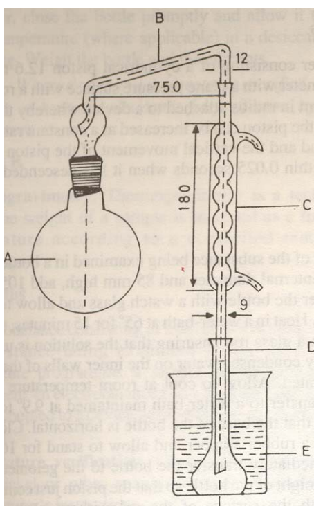
Fig.3 Apparatus for Determination of Ethanol by Distillation Method
