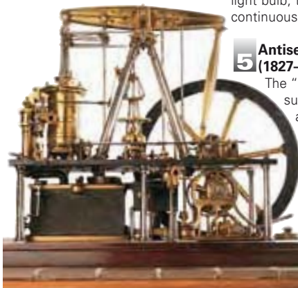
Rotative steam engine
