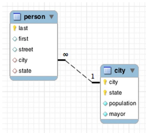
Figure 4-14. One-to-many relationship with natural keys
