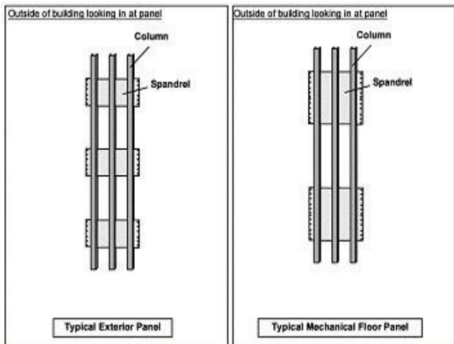
Figure 9-1 Spandrels – “Wheatchex” - Page 27 of NCSTAR1-3B
