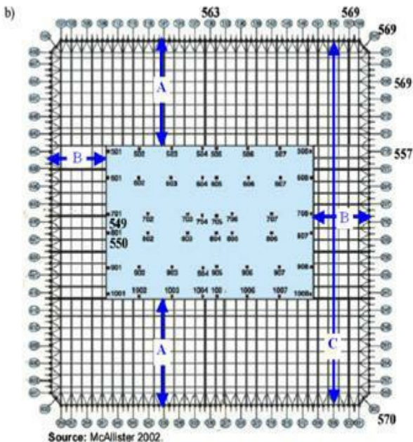
Figure 9-2 Diagram Illustrating Total Lengths of Truss Steel (Page 16 of NCSTAR1-3B)
